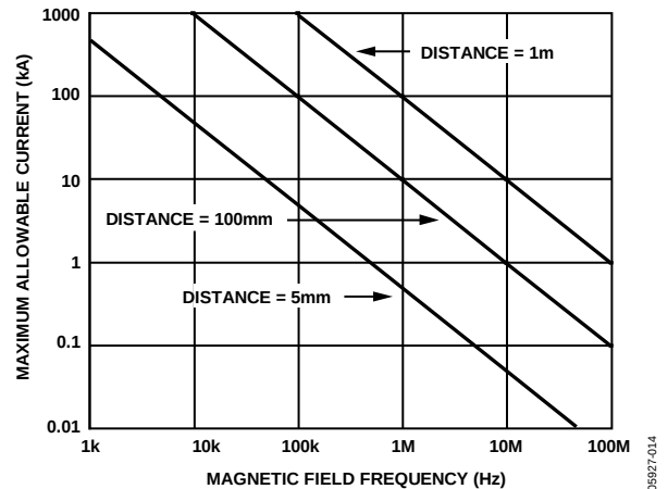
Figure 14. Maximum Allowable Current for Various Current-to-ADuM3200/ADuM3201 Spacing
